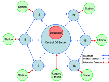
Figure 3. System architecture
